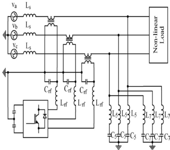
Fig. 2 SHAPF Topology Diagram
