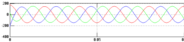
Fig.8 Load voltage with SHAPF
