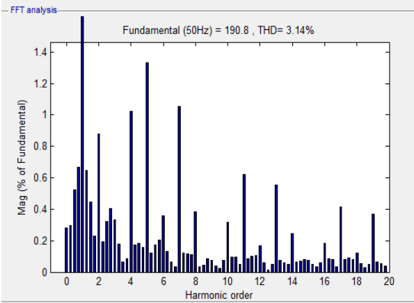
Fig. 7 THD Analysis with passive filter
