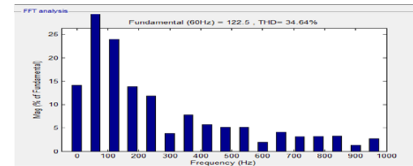
Fig. 4 THD Analysis without any filter
