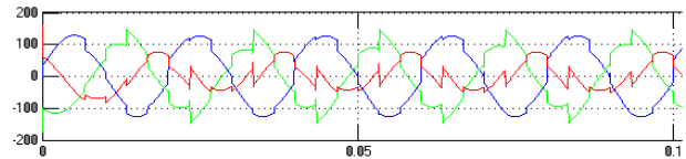
Fig. 2 Load voltage without any filter
