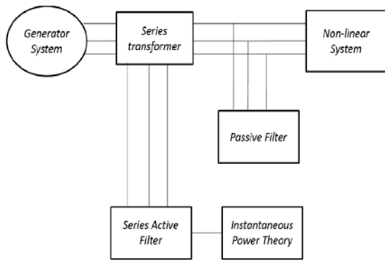
Fig. 1 Block Diagram of SHAPF
