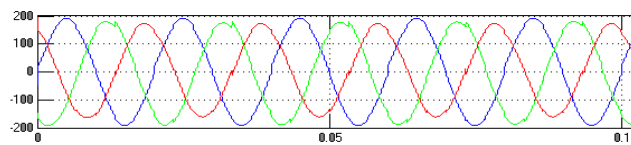
Fig. 5 Load voltages with passive filter
