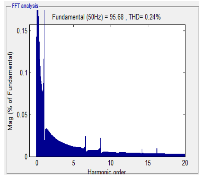
Fig. 10 THD Analysis with SHAPF
