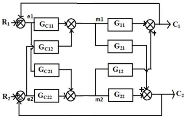
Fig.2. Closed loop block diagram of 2 X 2 systems
