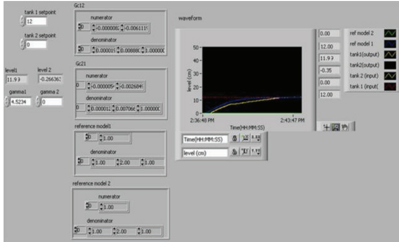
Fig.7.Response of the plant with Model Reference Adaptive Control for setpoint 12
