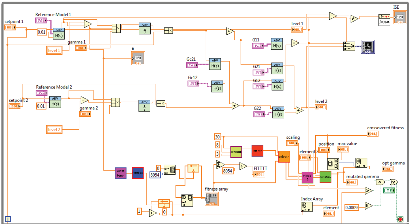
Fig.5. Block diagram of the plant with an optimised Model Reference Adaptive Control
