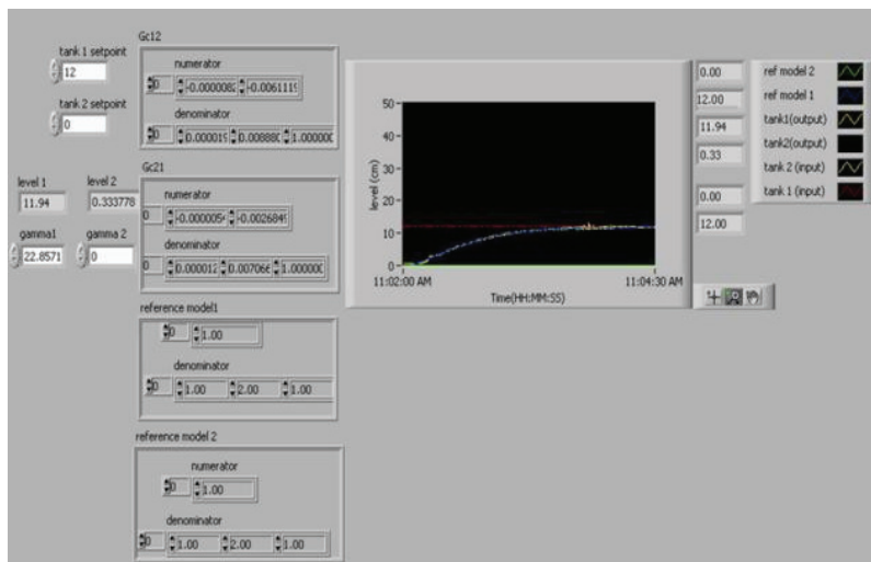
Fig.9.Response of the plant with an Optimised Model Reference Adaptive Control for setpoint 12
