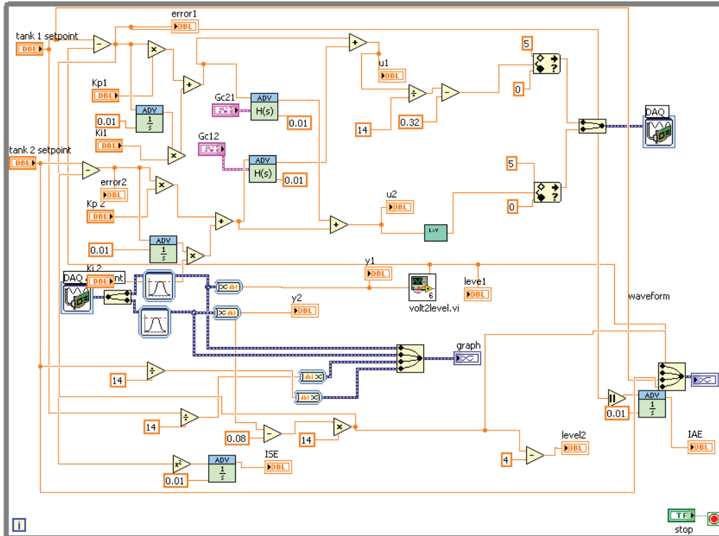
Fig.4. Block diagram of the plant with Model Reference Adaptive Control
