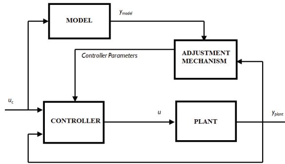
Fig.3. Block diagram of Model Reference Adaptive Control
