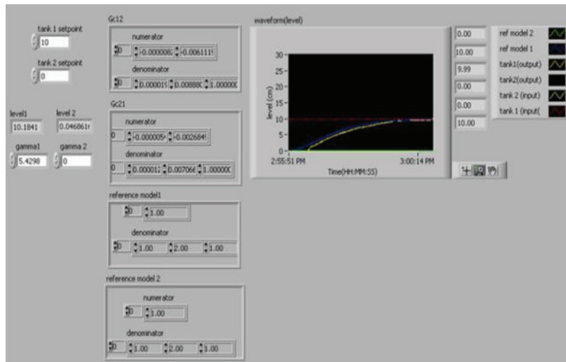
Fig.6. Response of the plant with Model Reference Adaptive Control for setpoint 10
