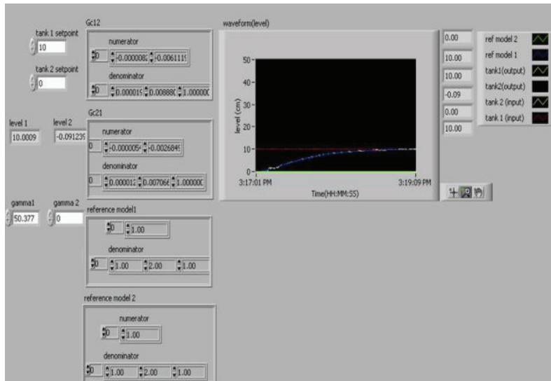
Fig.8.Response of the plant with an Optimised Model Reference Adaptive Control for setpoint 10
